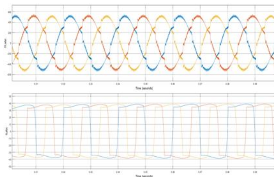
Figure 9 Load voltages and currents
