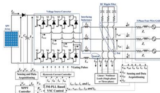
Fig. 4 Structure diagram of 3P4W grid-connected PV-ECS
