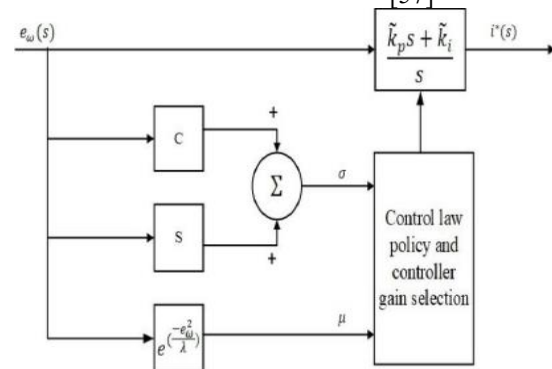
Figure 6 DSM-PI control scheme block diagram
