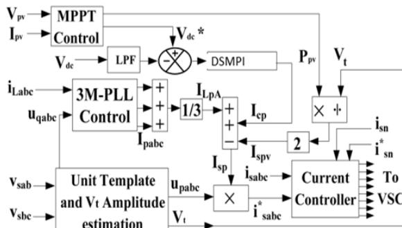
Fig. 5 Control scheme for 3P4W grid-tied PV-ECS
