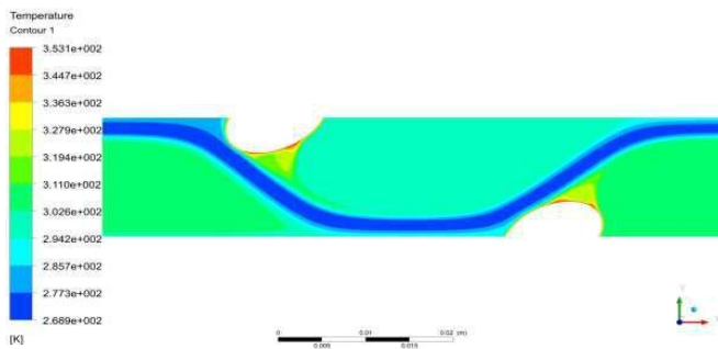
Figure 5: Temperature distribution over the plate fin with elliptical tube inclined at 30^\circ heat exchanger
