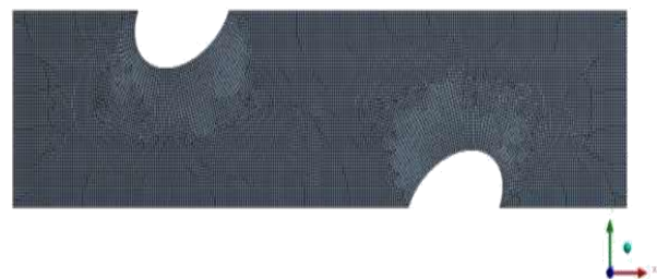
Figure 4. Meshing of plate fin with elliptical tube inclined at 30° heat exchanger
