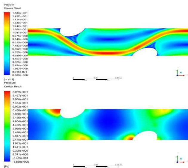
Figure 6 Velocity distribution over the plate fin with elliptical tube inclined at 30^\circ heat exchanger
