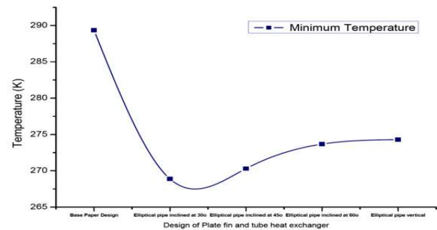
Figure 7: Minimum Temperature Distribution over the plate fin tube heat exchanger
