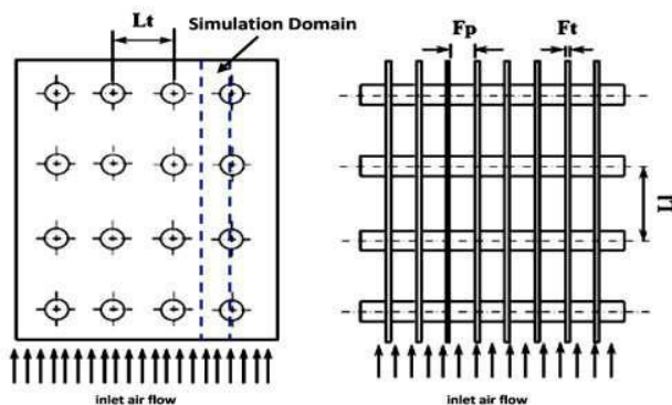
Figure 1: Physical model with staggered arrangement
