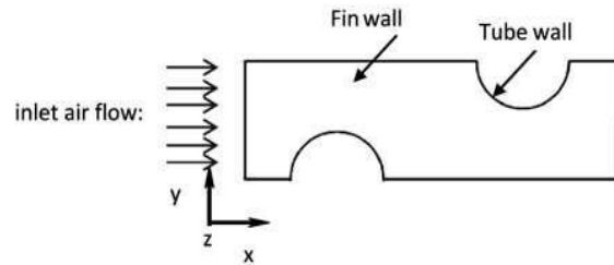
Figure 2: computational domain with different boundaries of fin tube heat exchanger
