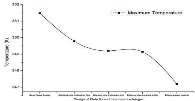
Figure 8: Maximum Temperature Distribution over the plate fin tube heat exchanger
