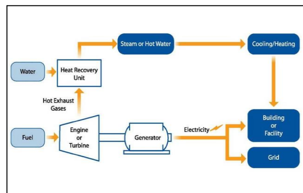
Figure 1: CHP Process Flow Diagram
