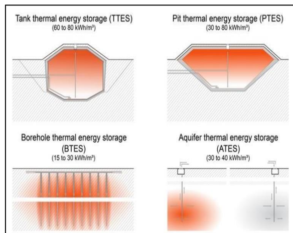
Figure 2: Types of Large-Scale Sensible thermal storage systems
