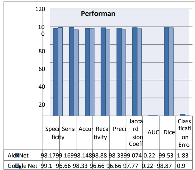
Figure 5 performance comparisons of deep learning models
