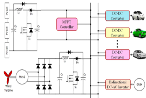
Fig.4. Implementation of the proposed charging station
