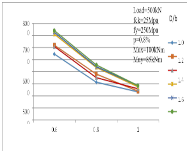
Fig. 1 Cost for a percentage of steel of 0.8%
