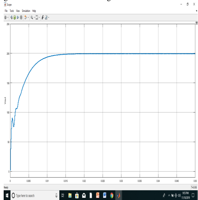
Fig. No. 4 Output voltage for high step up converter with R load
