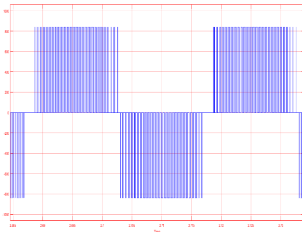
Fig. 6 Inverter voltage of phase A
