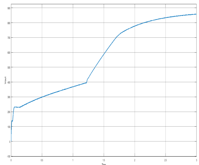
Fig. 5 DC voltage output of the proposed converter when connected to induction machine
