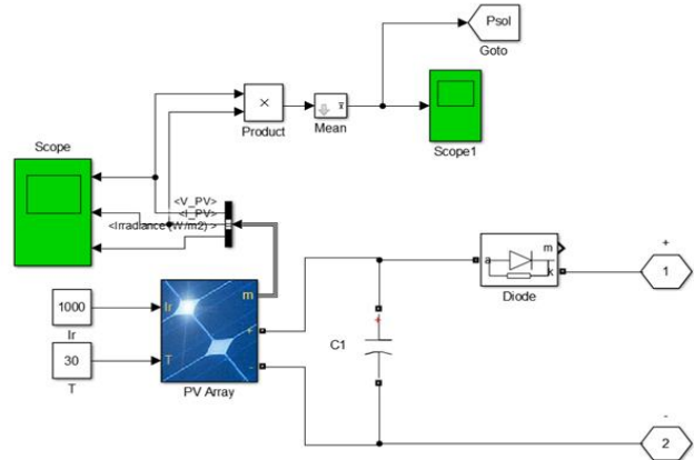
Figure 7: PV module internal modelling
