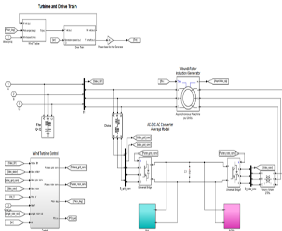
Figure 6: DFIG internal modeling
