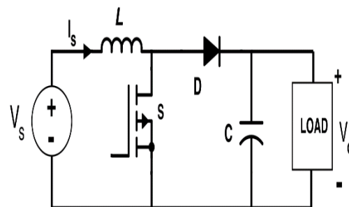
Figure 4: Boost converter Schematic
