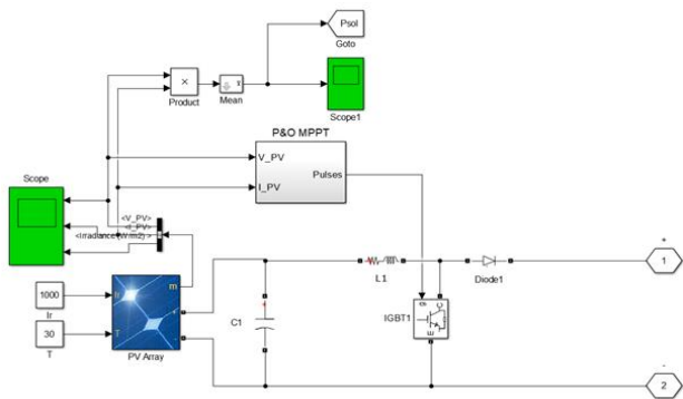
Figure 9: Modified PVA module with DC-DC booster converter
