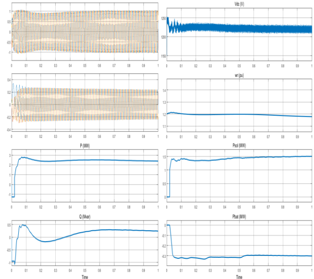
Figure 8: Generated results of the proposed system
