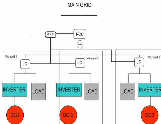
Figure 1: Block diagram of Microgrid
