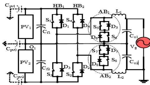
Figure 2 model of grid connected transformer-less inverter Controlling PV arrays
