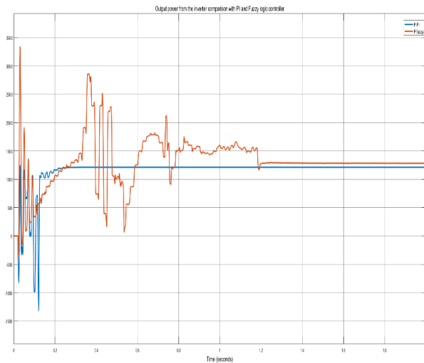
Figure 7 Output power from the inverter comparison
