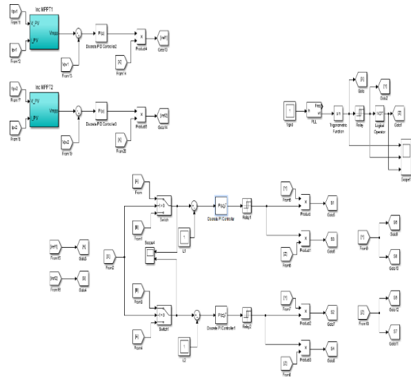
Fig.4 Proposed control structure modelling
